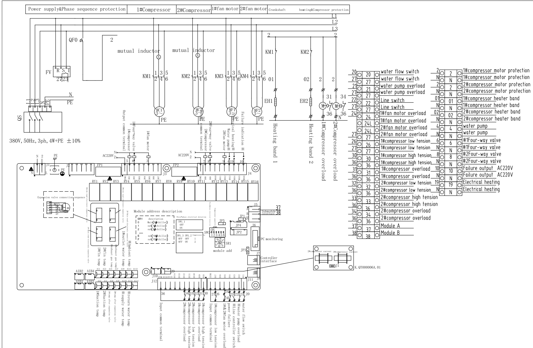
Electric diagram Model: EMACO-440.V2
